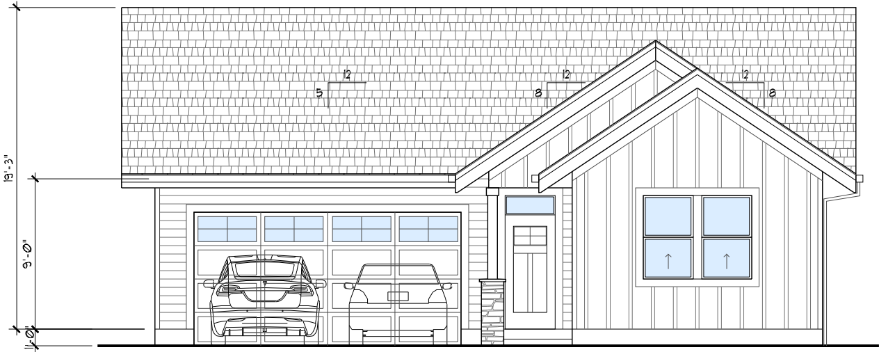
UNIT 1 - ELEV C
